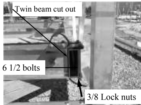
View of winch column area end view of the winch cable tube.
