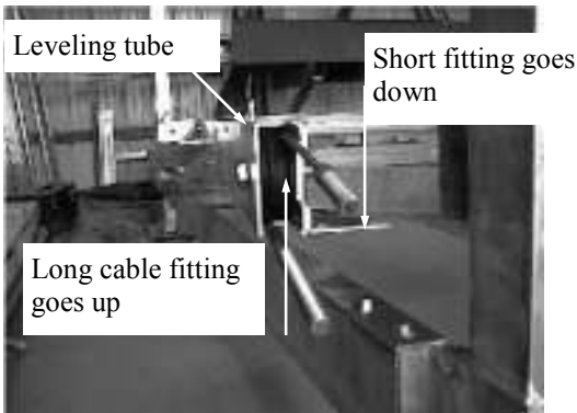
Non winch front side of hoist.
