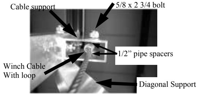
View of winch side, rear corner of hoist.
