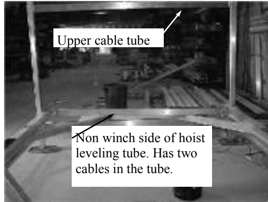
Lay the leveling tube on the non winch side of the hoist. In between the twin beams. See below for close up photos of the tube and how it is positioned on the hoist.
