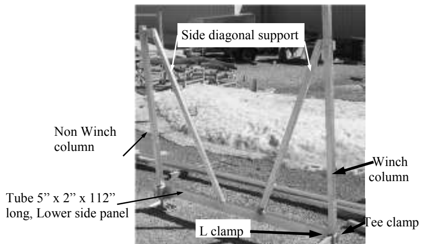
View of non winch side panel
