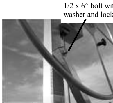
Close up of winch column brace connection.
